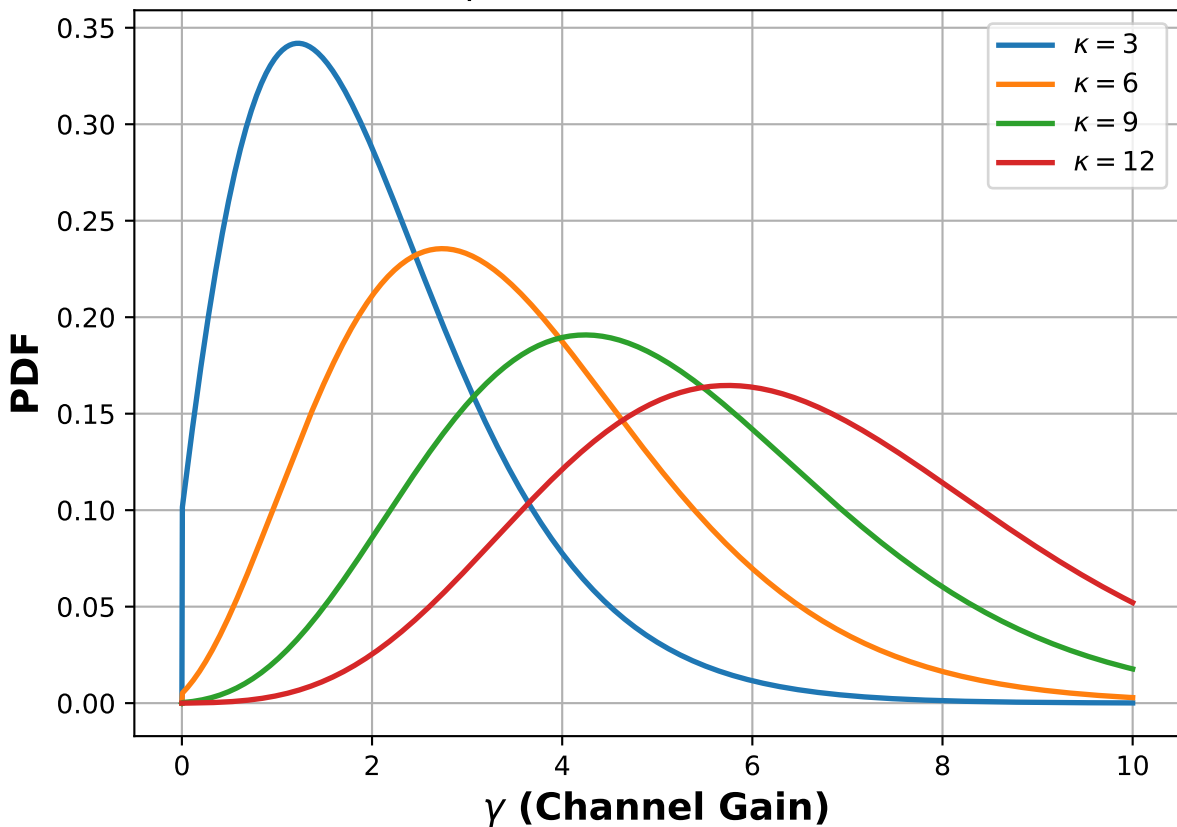
PDF of \gamma with d=2.0 , N_t=1 (SISO)
